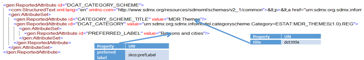
Figure 29: SDMX category scheme metadata pertaining to the DCAT-AP Catalogue
