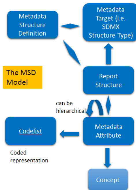
Figure 24: Schematic diagram of the SDMX Metadata Structure Definition model
