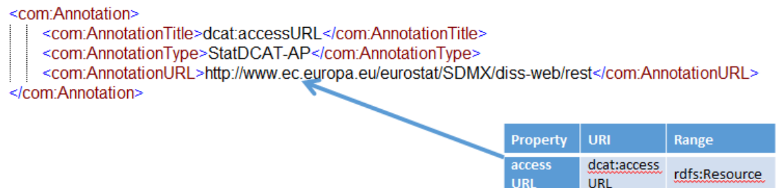
Figure 22: Transformation format - Linking a Distribution (accessURL) to the SDMX Provision Agreement
