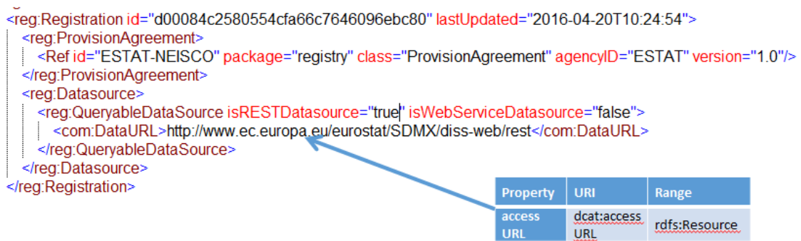
Figure 21: From Section 9 - Linking a Distribution (accessURL) to the SDMX Provision Agreement
