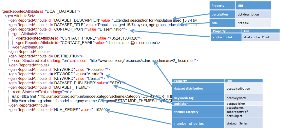
Figure 30: SDMX dataset metadata pertaining to the DCAT-AP Catalogue including StatDCAT-AP extensions to the Dataset.
