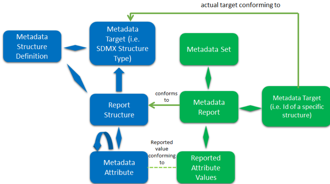
Figure 25: Schematic diagram of the SDMX Metadata Set
