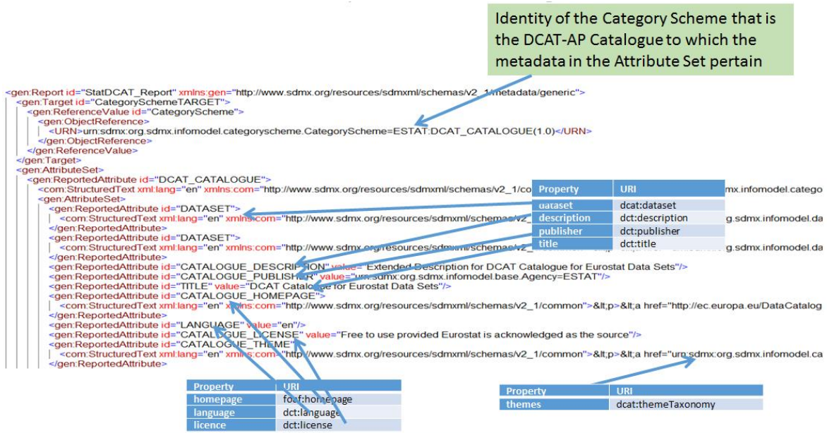
Figure 28: SDMX catalogue metadata pertaining to the DCAT-AP Catalogue
