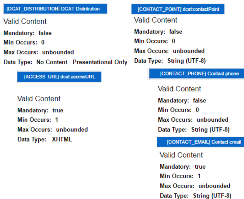
Figure 27: Example of Metadata Attribute Specification
