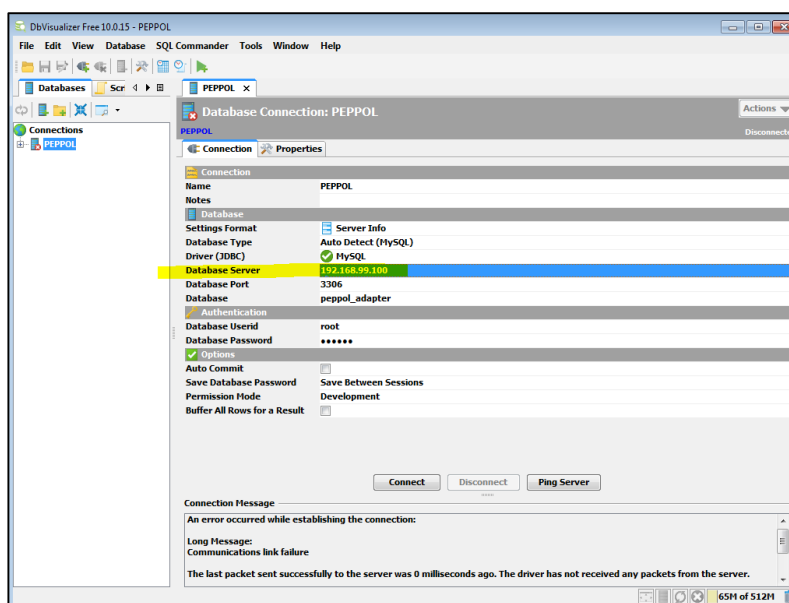
Fig. 10. Database connection properties
