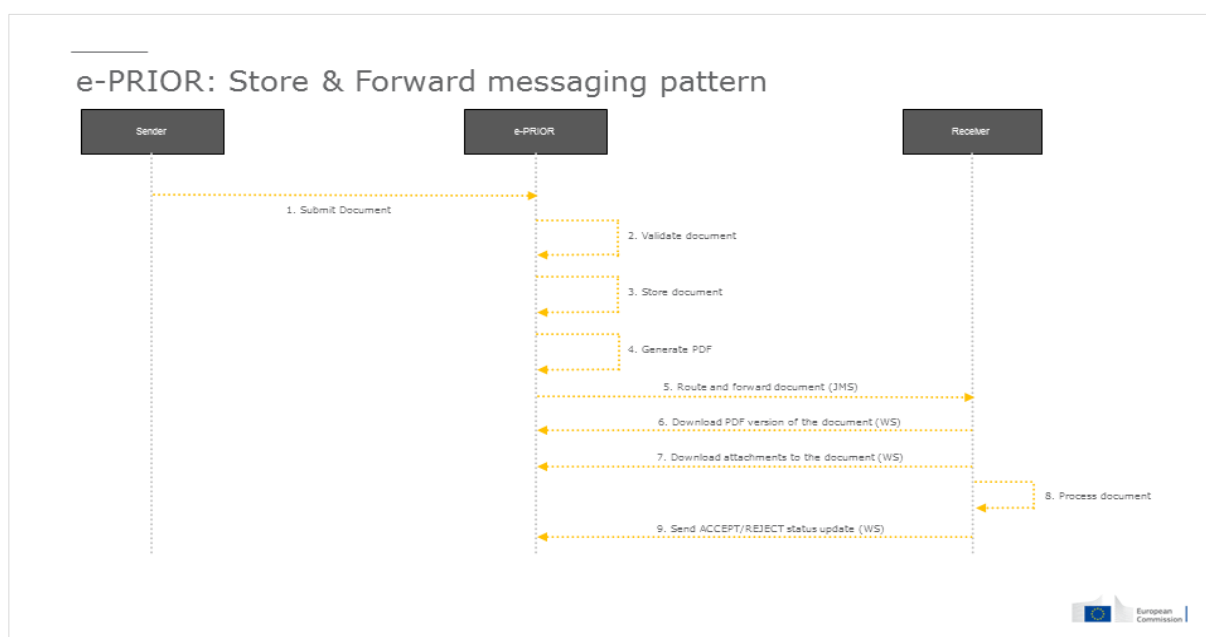
Fig. 28. Store&Forward integration pattern
