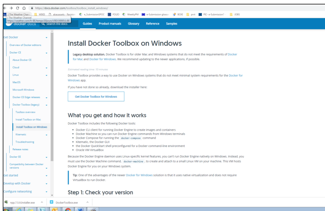
Fig. 5. Docker Installation
