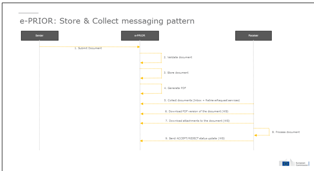
Fig. 29. Store&Collect integration pattern
