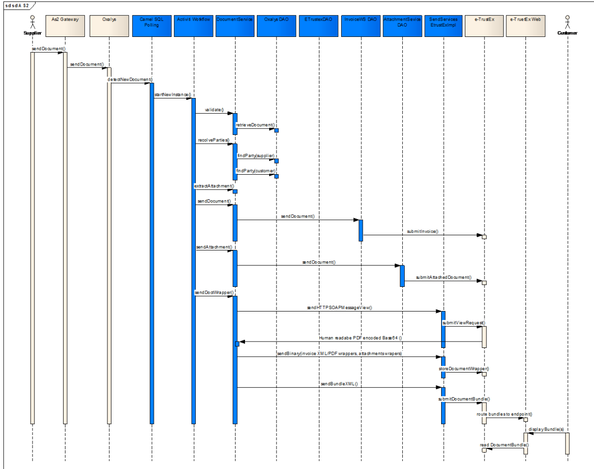
Fig. 4. Sequence diagram
