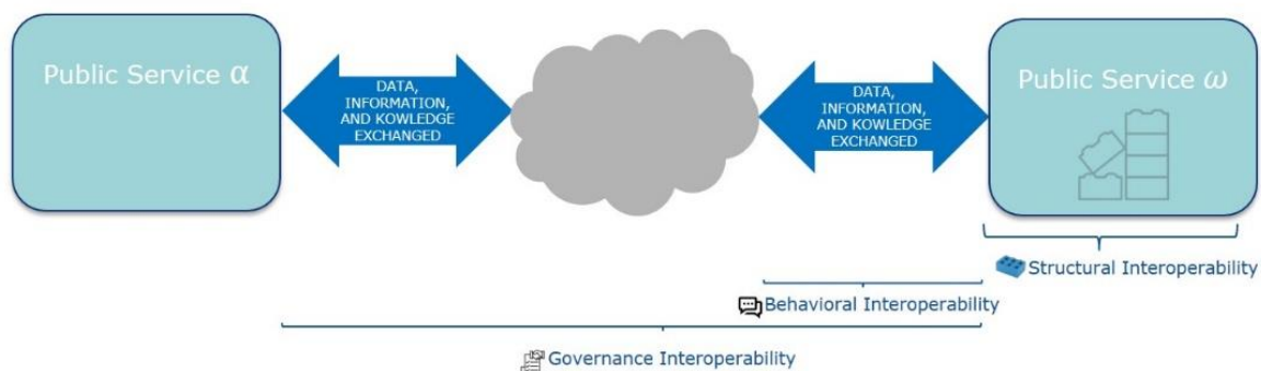
Figure 1: Interoperability dimensions
