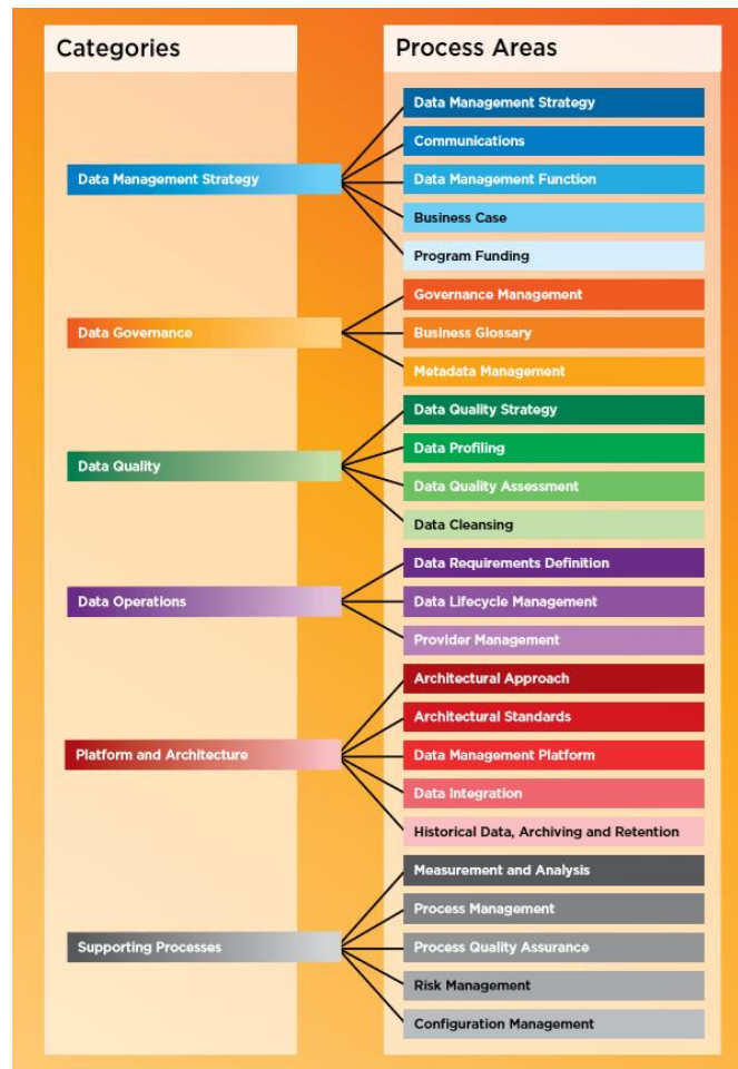
Figure 4: CMMI – DMM Process areas 31
